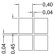
Dots Detail
